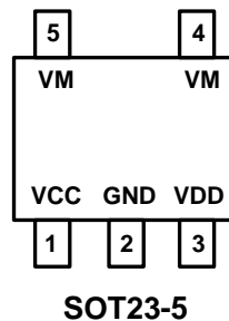
Figure 2. PIN Configuration
