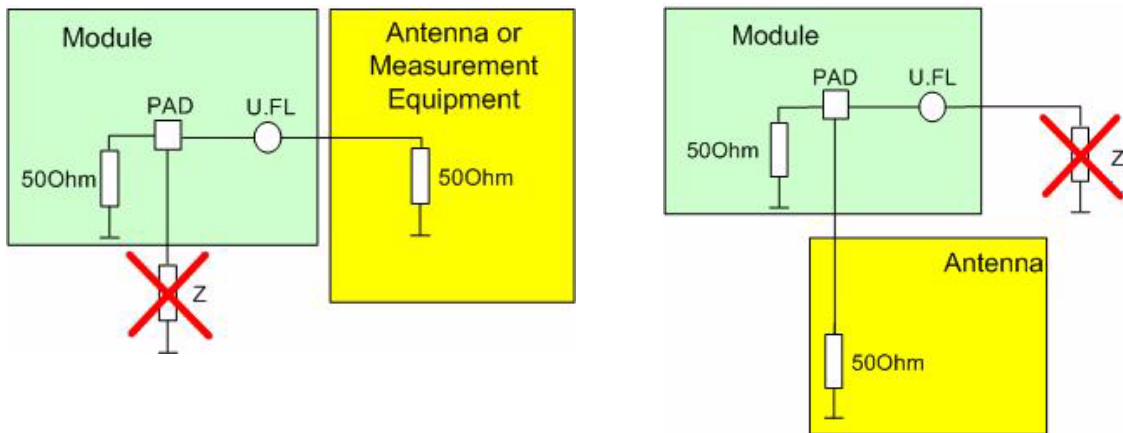
Figure 26: Never use antenna connector and antenna pad at the same time
