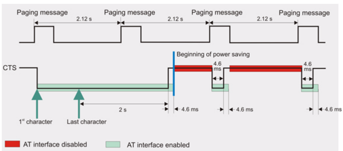
Figure 11: Beginning of power saving if CFUN=5 or 7
