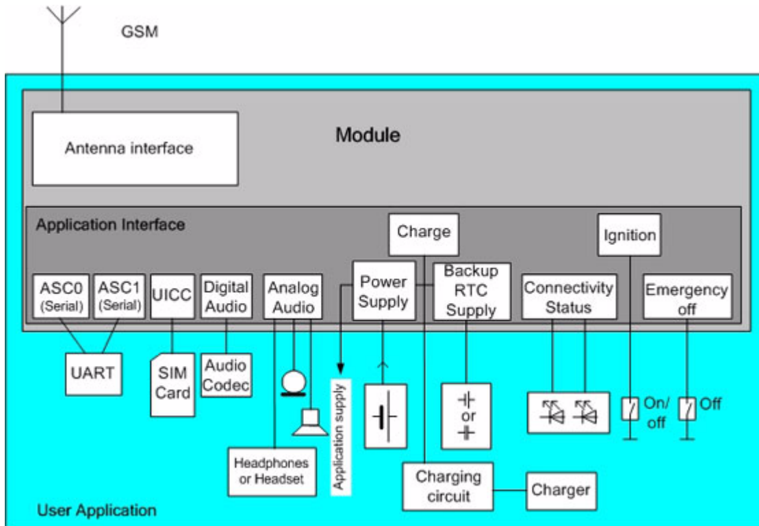
Figure 1: MC55i system overview
