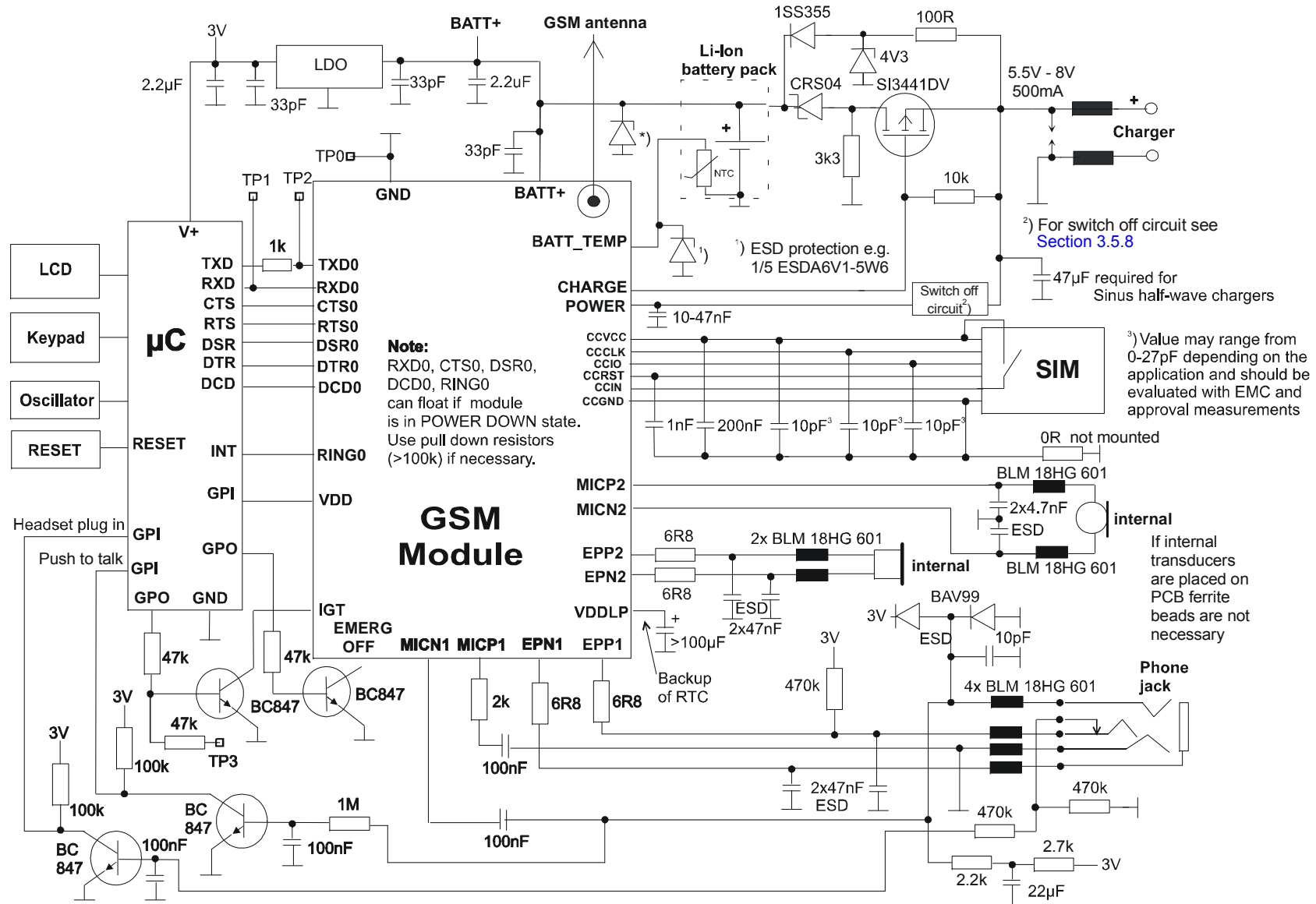
Figure 40: Schematic diagram of MC55i sample application
