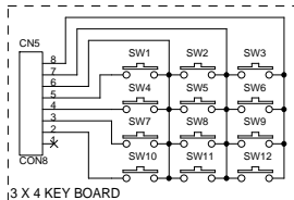
3 X 4 KEY BOARD
